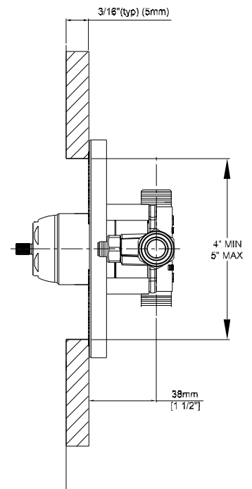
THIN WALL
