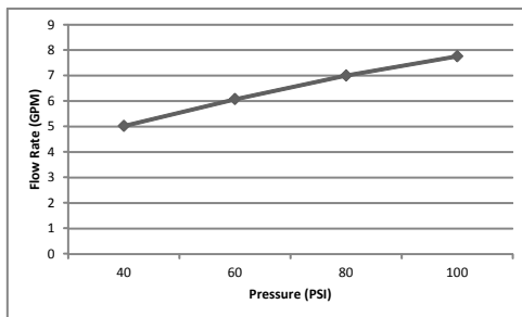
P-2303B Flow Rate (GPM) Vs Pressure (PSI) For Tub Port*
