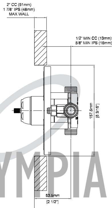
THICK WALL
