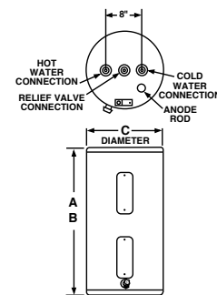
WATER CONNECTIONS ALL 3/4" N.P.T.
